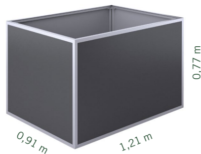
ALUMINIUM-HOCHBEET 130
