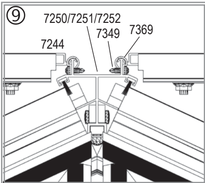
ADDITIONAL ROOF VENT Z2
