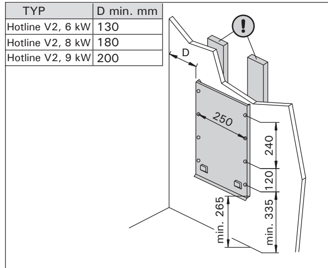
Figure 7. Location of the mounting rack of the heater (all dimensions in millimeters)
