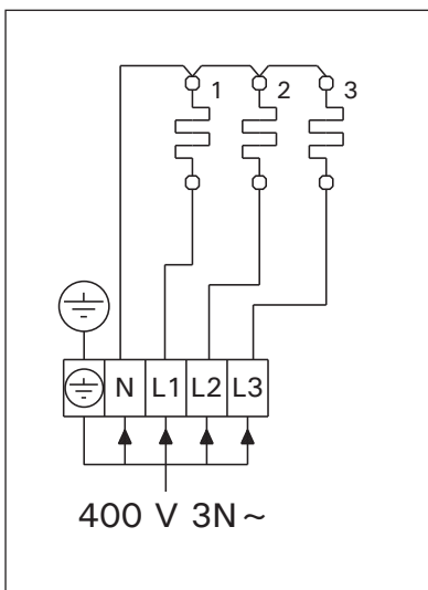
Figure 9. Electrical connections of heater Abbildung 9. Elektroanschlüsse des Saunaofens
