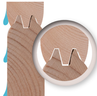
38mm PROFILE
