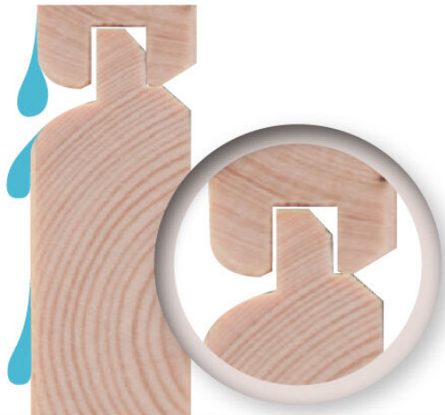
19mm PROFILE
