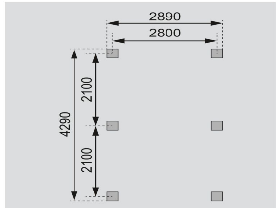
Fundamentplan Pfosten (in mm)
