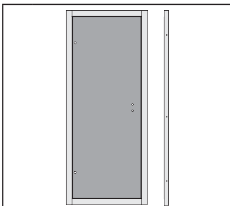
1 x W5 1872 x 750 x 68 mm ID 43454
