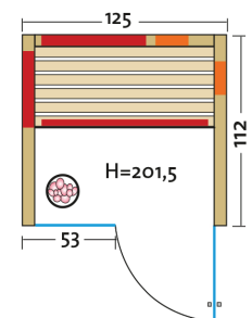
Detail Tannenholz
