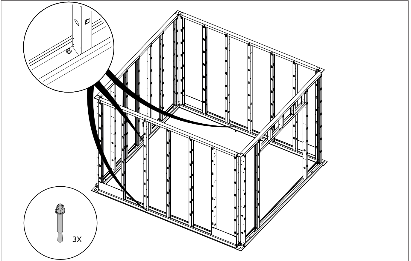
A/B/C/D Ancrage / Verankering / Anchoring / Verankerung
